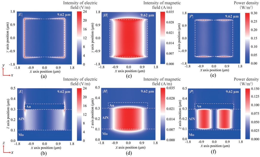
Fig. 2 Mapping of electric and magnetic field distributions at MAs absorption peak; (a) x - y plane and (b) x - z plane electric field distributions; (c) x - y plane and (d) x - z plane magnetic field distributions; (e) x - y plane and (f) x - z plane power density distributions 图2 MAs吸收响应处的电场和磁场分布图:(a) x - y 平面和(b) x - z 平面电场分布;(c) x - y 平面和(d) x - z 平面磁场分布;(e) x - y 平面和(f) x - z 平面功率密度分布
