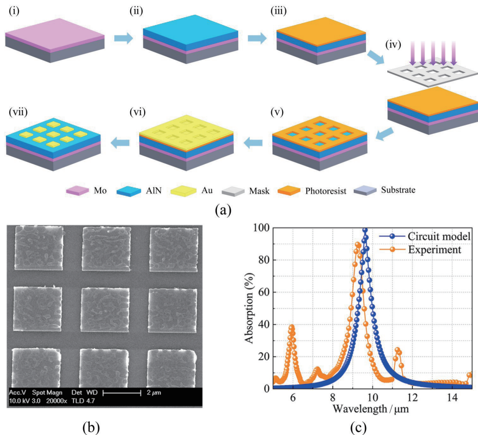
Fig. 5 Preparation by MIM-MAs process: (a) process steps for fabrication of MAs; (b) SEM image of the fabricated MAs; (c) tested MAs absorption response (orange points) versus the absorption response predicted by the RLC equivalent circuit model (blue points) 图5 MIM-MAs工艺制备:(a)制备MAs工艺步骤;(b)所制备MAs的SEM图像;(c)测试MAs的吸收响应(橙色)与RLC等效电路模型预测的吸收响应(蓝色)对比
