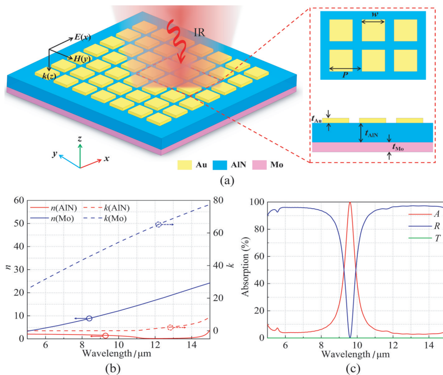
Fig. 1 MIM-MAs infrastructure and related performance: (a) schematic of the proposed structure of MIM-MAs; (b) optical parameters of AlN and Mo; (c) absorption, reflectivity and transmittance curves of the MAs structure
