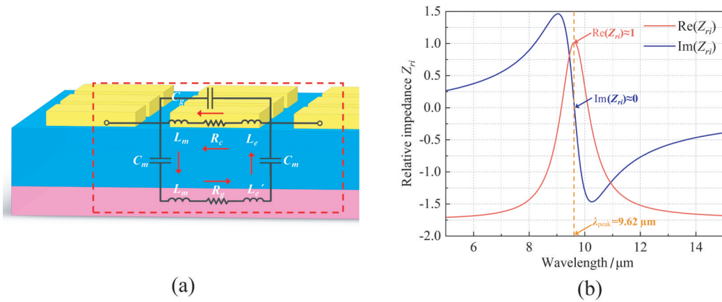
Fig. 3 Proposed equivalent circuit model structure: (a) schematic diagram of the RLC equivalent circuit model for MIM-MAs; (b) real and imaginary parts of the relative impedance of the equivalent circuit model 图3 等效电路模型结构:(a) MIM-MAs结构等效电路模型示意图;(b)等效电路模型相对阻抗的实部和虚部
