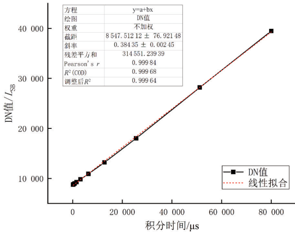
图 17 黑体响应与积分时间线性度的关系 Fig. 17 Relation between blackbody response and integration time linearity
