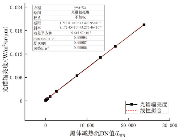
图 18 黑体响应与光谱辐亮度线性度的关系 Fig. 18 Relation between blackbody response and spectral radiance linearity
